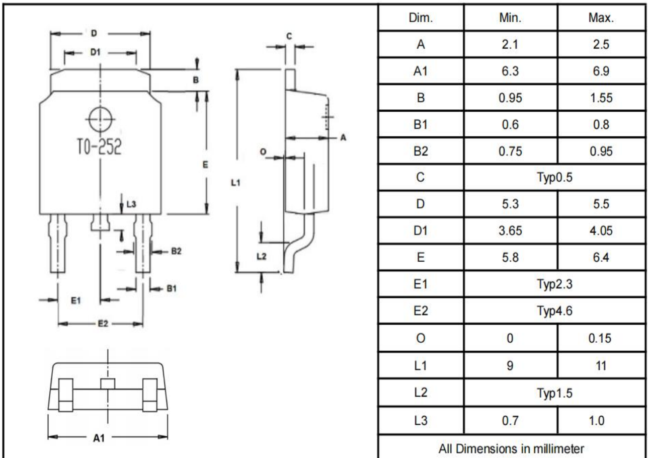
TO-252
