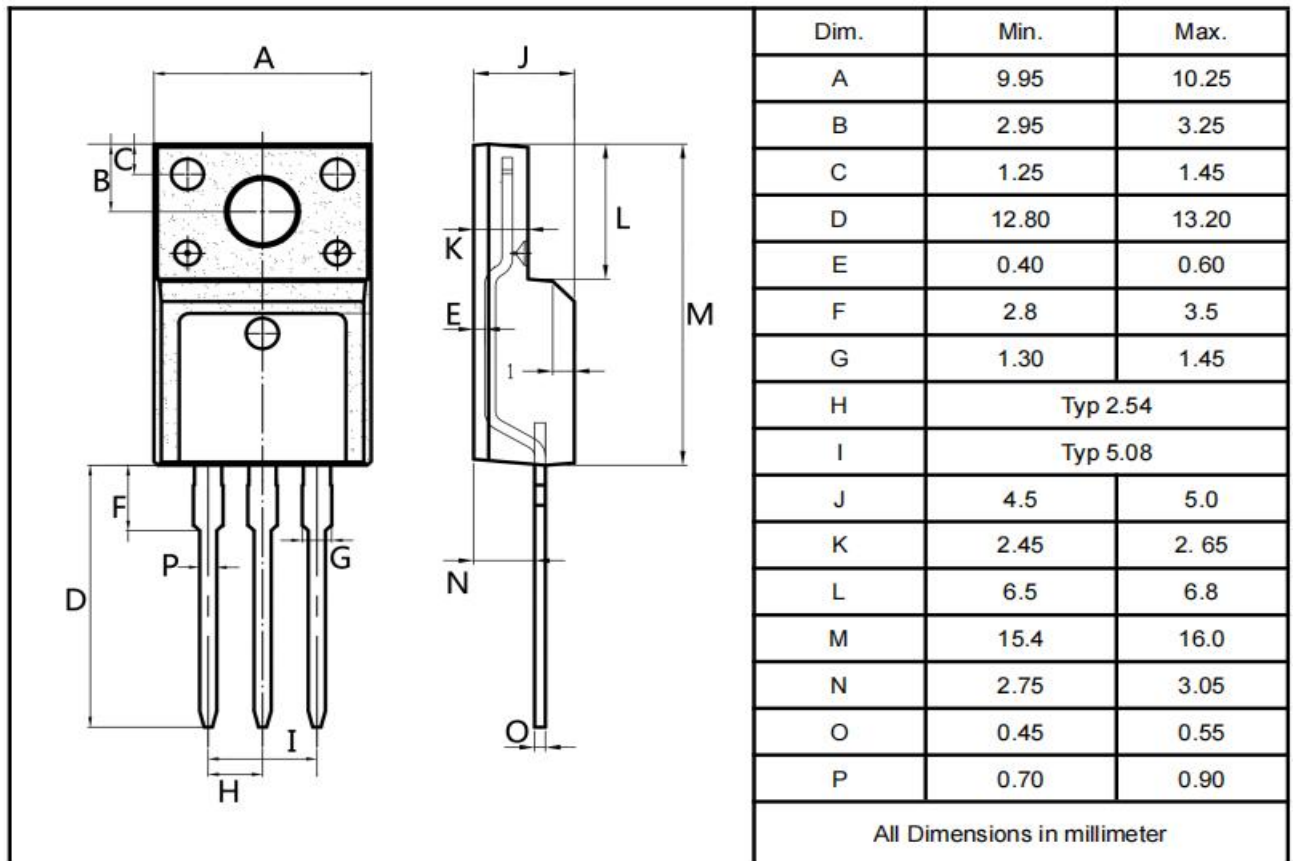
TO-220F
